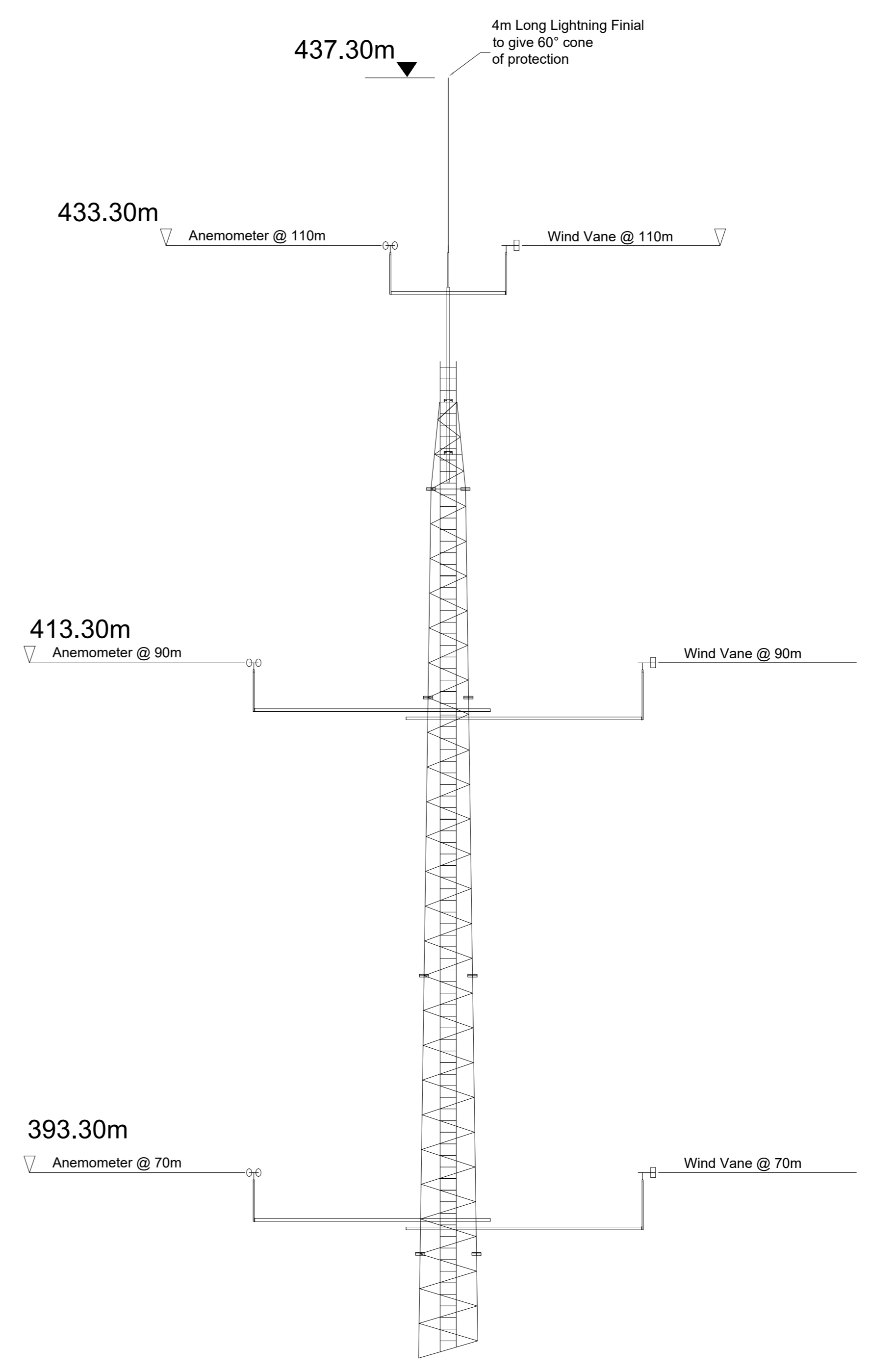
ANEMOMETER & WIND VANE LOCATIONS
