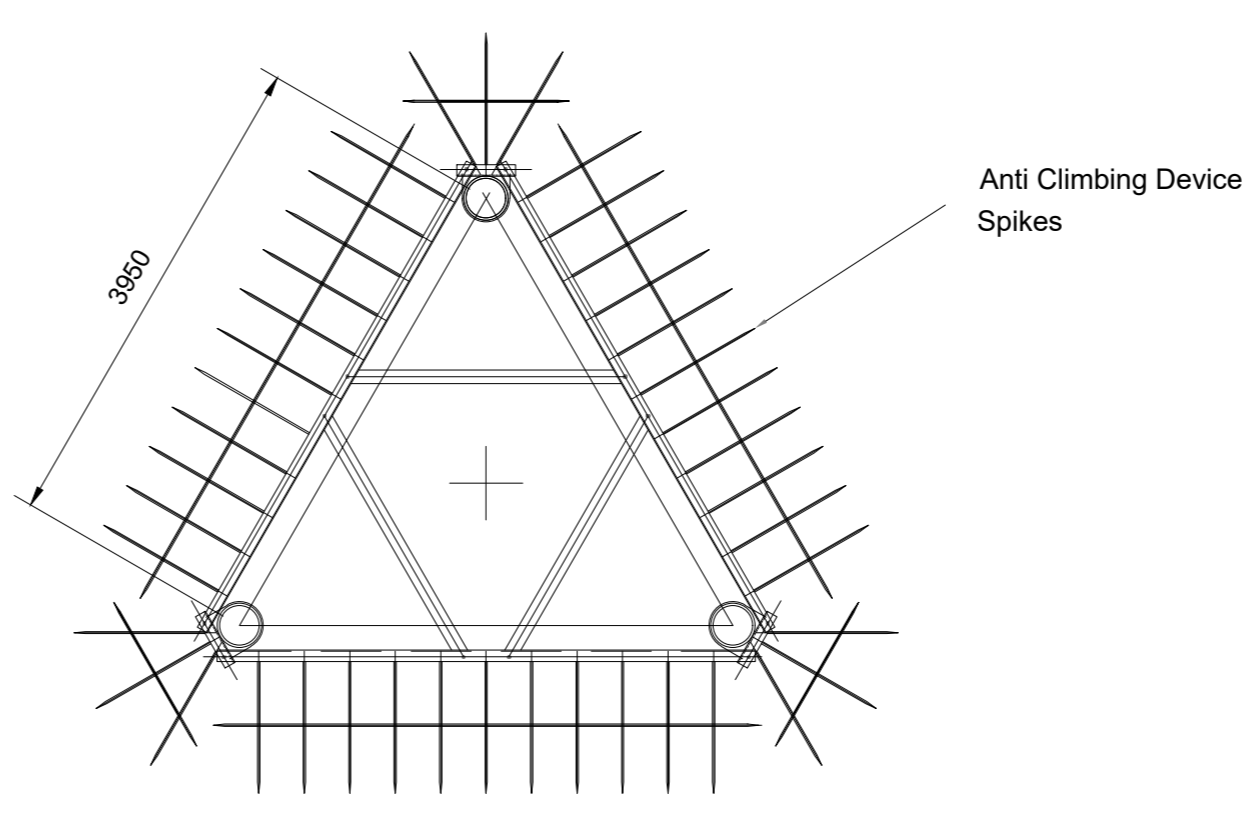
ANTI CLIMBING DEVICE
