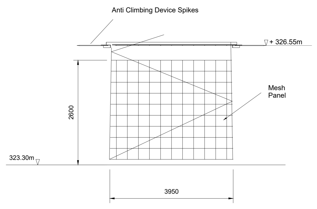
SECURITY PANEL TO BASE OF TOWER
